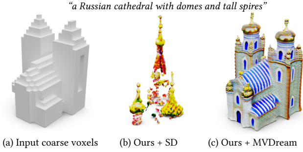
Fig. 6. Ablation study on the choice of image diffusion models. (a) We train both models with the same coarse input in the first stage. (b) Our method with a single-view diffusion model (Stable Diffusion) as SDS guidance struggles to produce a complete shape. (c) Our method with a multi-view diffusion model (MVDream) as guidance produces high-quality results.
