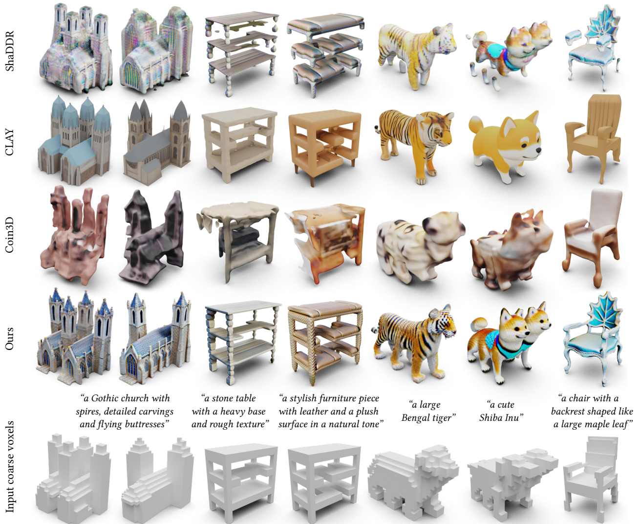
Fig. 14. Qualitative comparison of text-guided detailization with input coarse voxels control. Note that even with a simple structure, as shown in the last column, existing methods fail to produce plausible results when given a creative text prompt.
